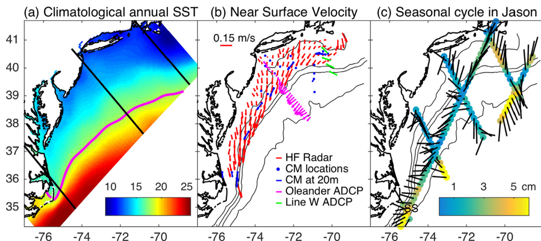
Fig. 2. Observations used in the assimilation and validation. (a) Annual mean sea surface temperature from MOCHA climatology. Solid black lines define northern and southern sub-regions of MAB, and the purple line (18 °C isotherm) the extent of the Slope Sea, used in averages in subsequent figures. (b) Annual mean surface velocity from HF Radar averaged in 30 km bins (red arrows), 20-m depth velocity from current meters (blue arrows), and 35-m depth velocity from Oleander ADCP (magenta arrows) and Line-W (green arrows). Blue dots indicate current meters reporting at other depths. (c) Seasonal cycle amplitude (colored circles) and phase (orientation of black lines) for along track Jason altimeter observations. Phase advances clockwise from north starting January 1. Thin black lines in (b) and (c) are 50, 200, 1000 and 3000 m isobaths. (For interpretation of the references to color in this figure legend, the reader is referred to the web version of this article.)
