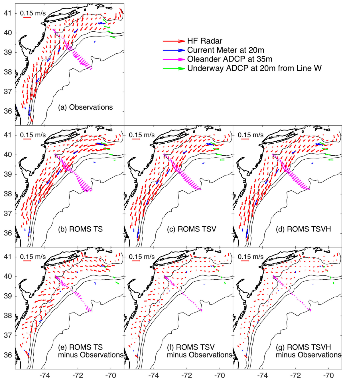
Fig. 5. Comparison of annual mean velocity from ROMS TS, TSV and TSVH experiments with measured velocity from HF-radar (red arrows), 35-m depth Oleander ADCP (magenta arrows), current meter at 20m depth (blue arrows), and Line-W ADCP at 20m depth (green arrows). Thin black lines show 50, 200, 1000 and 3000 m isobaths. Model velocities are interpolated to the same locations as observations and shown in the same color. (For interpretation of the references to color in this figure legend, the reader is referred to the web version of this article.)
