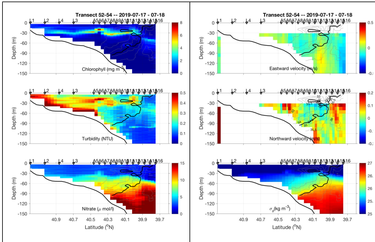
Figure 0718.2. July 17-18 CTD transect. Note labeling of stations L3 and L4 are backward.
