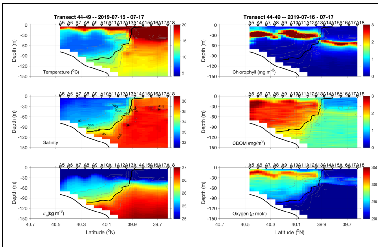
Figure 0717.1. July 16-17 CTD transect.
