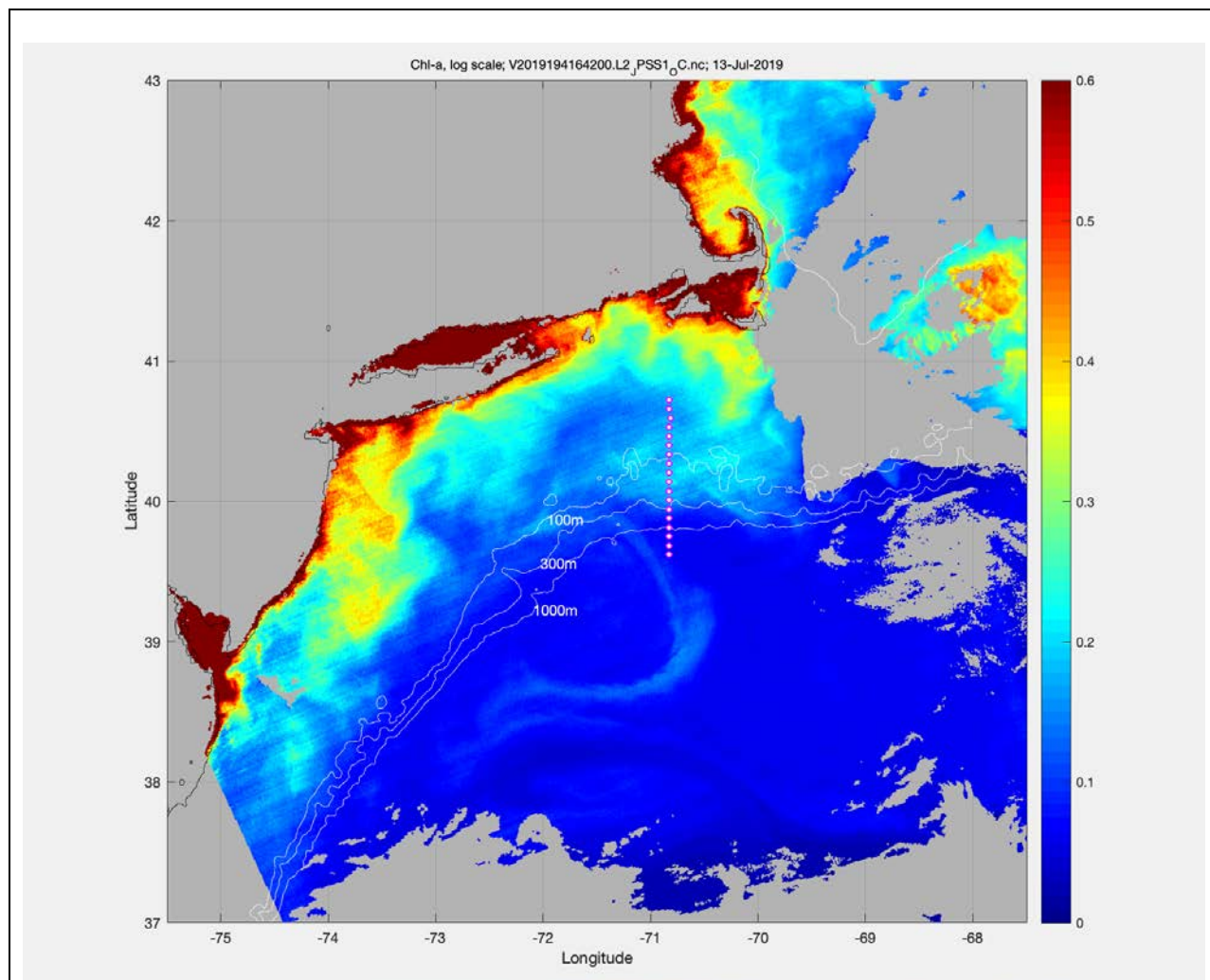
Figure 0713.5. VIIRS chlorophyll on July 13.
