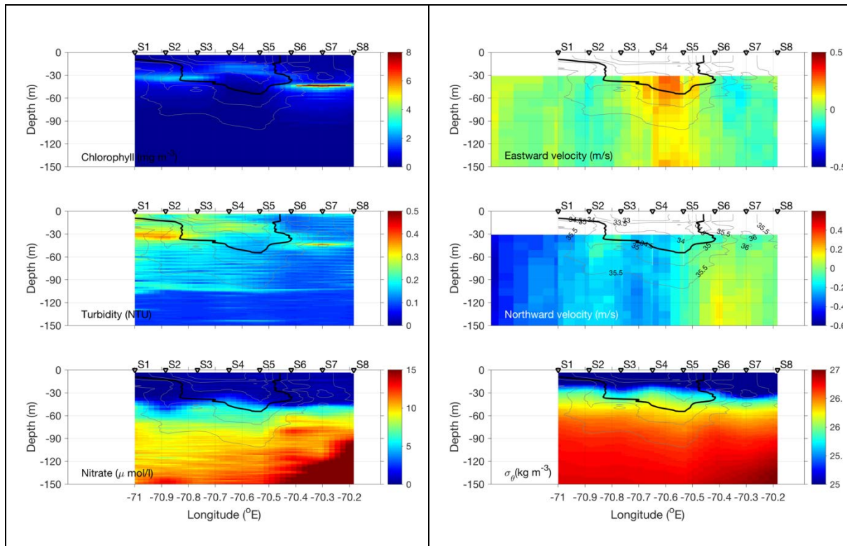
Figure 0708.4. July 8 streamer transect 0-150m.
