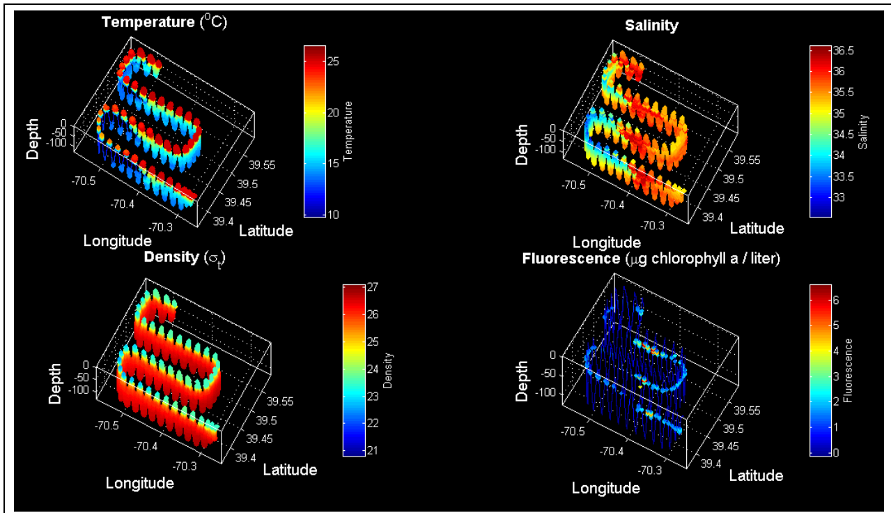
Figure 0710.5. VPR4 July 10-11, starting from station SSF6 in the streamer/slope front section (Figure 0709.1,2).
