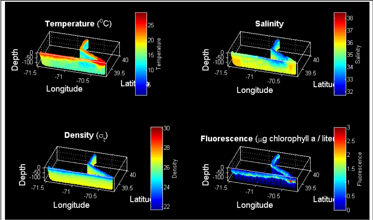
Figure 0708.1. VPR2 survey of ring streamer.
