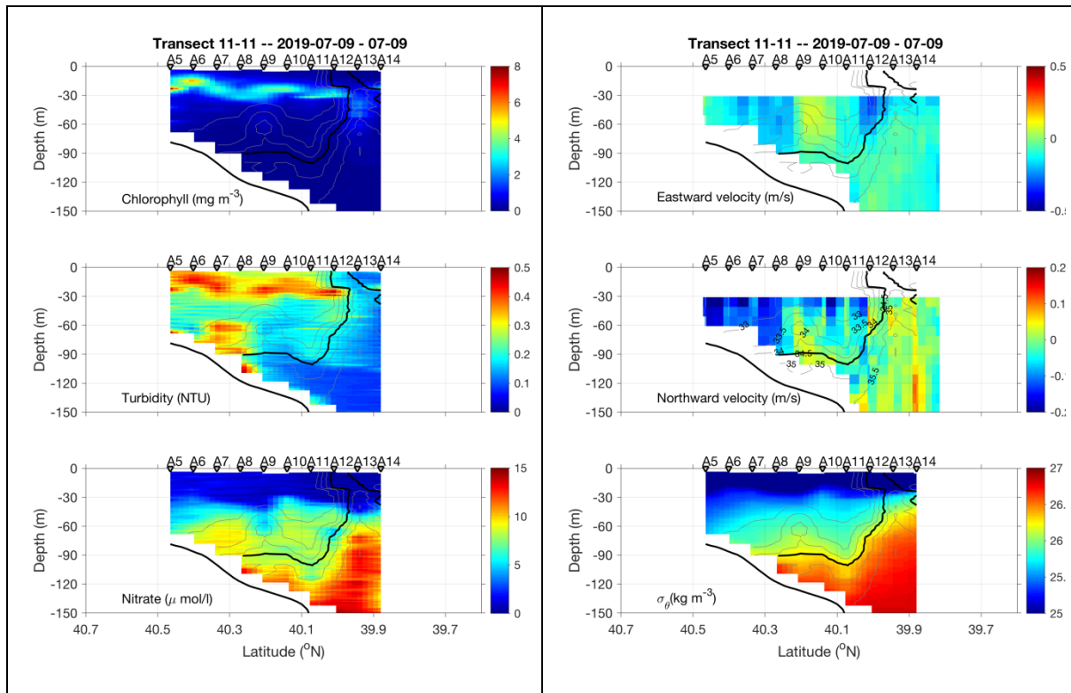
Figure 0709.2. July 9 CTD transect 0-150m.
