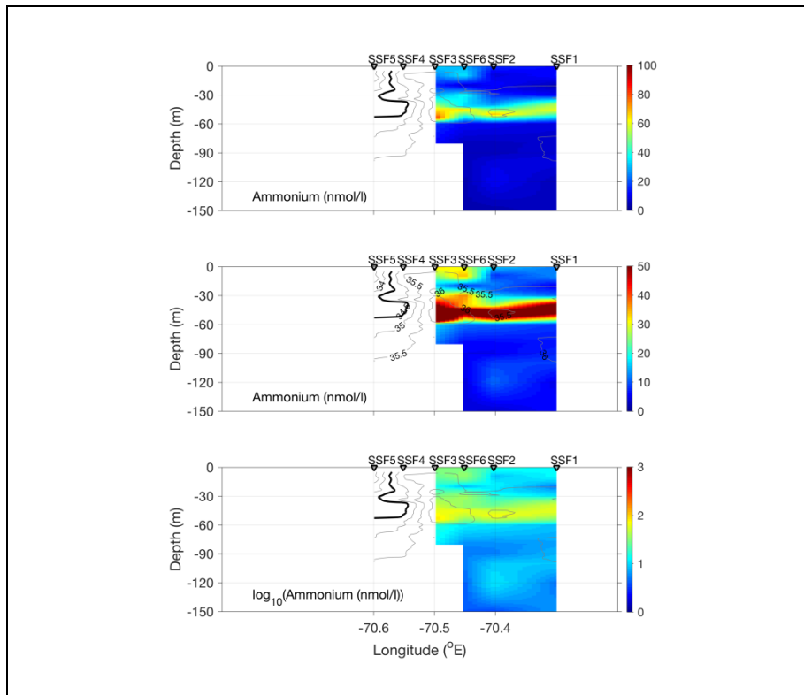
Figure 0710.3. July 10 CTD transect across the streamer/slope front.
