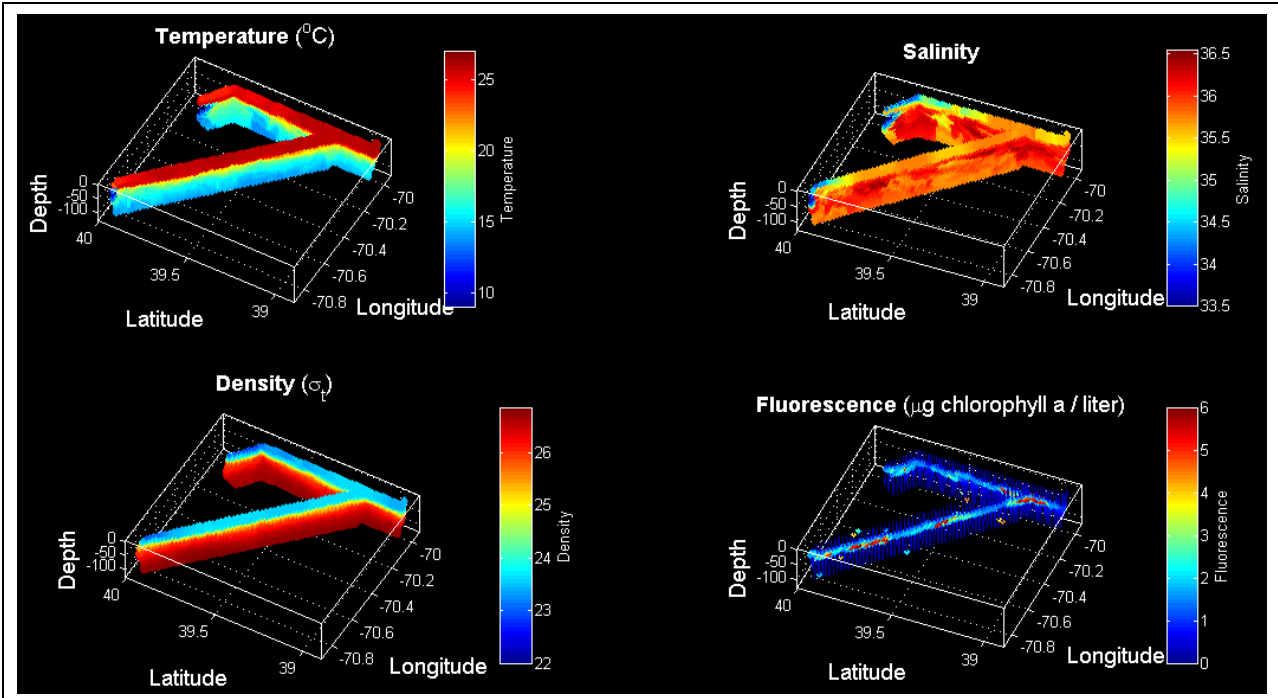
Figure 0715.5. Combined VPR7/8 survey on July 14-15.
