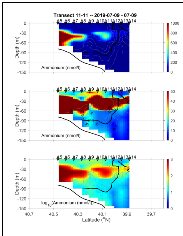
Figure 0709.3. July 9 CTD transect 0-150m.
