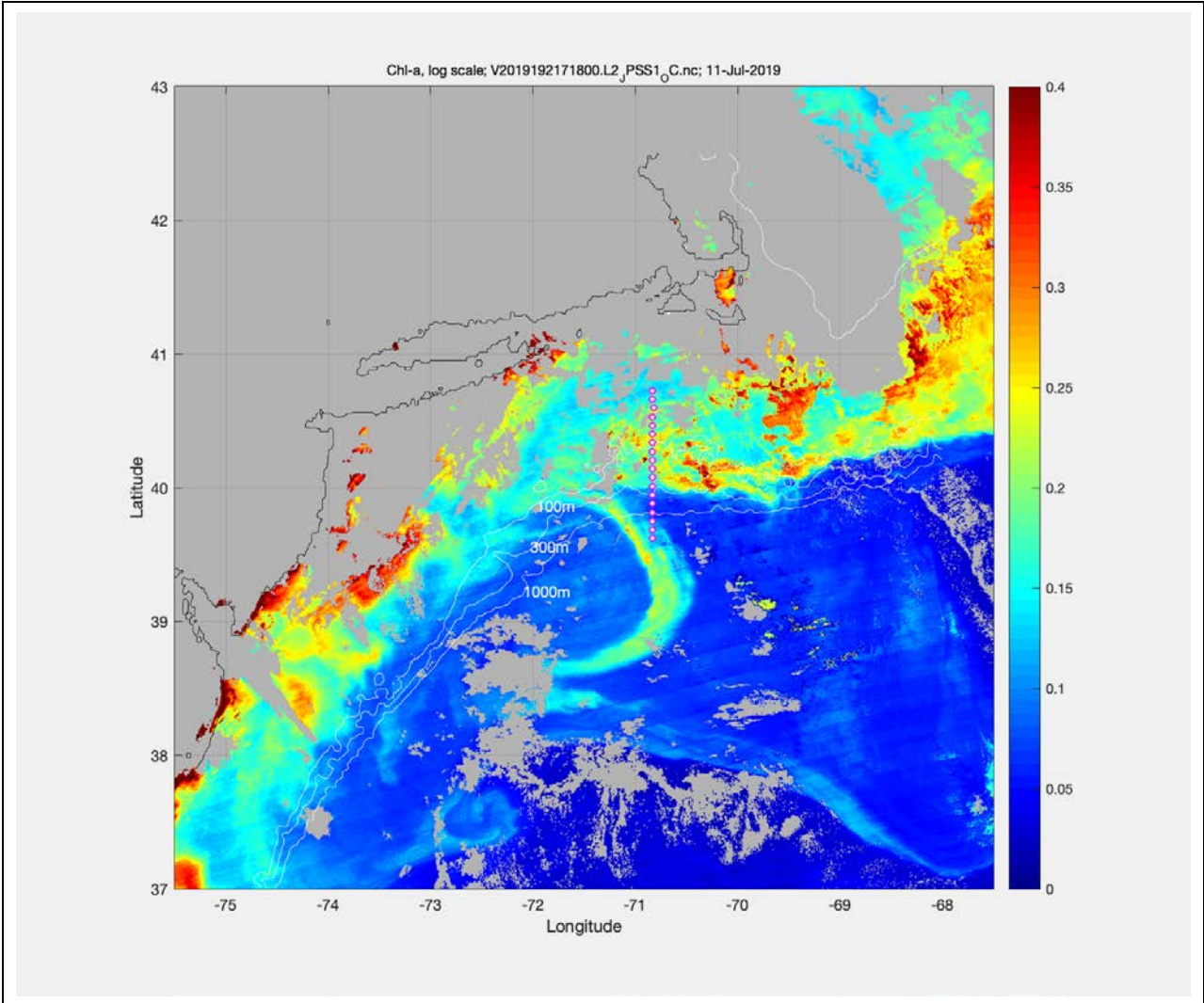
Figure 0713.3. VIIRS chlorophyll on July 11.
