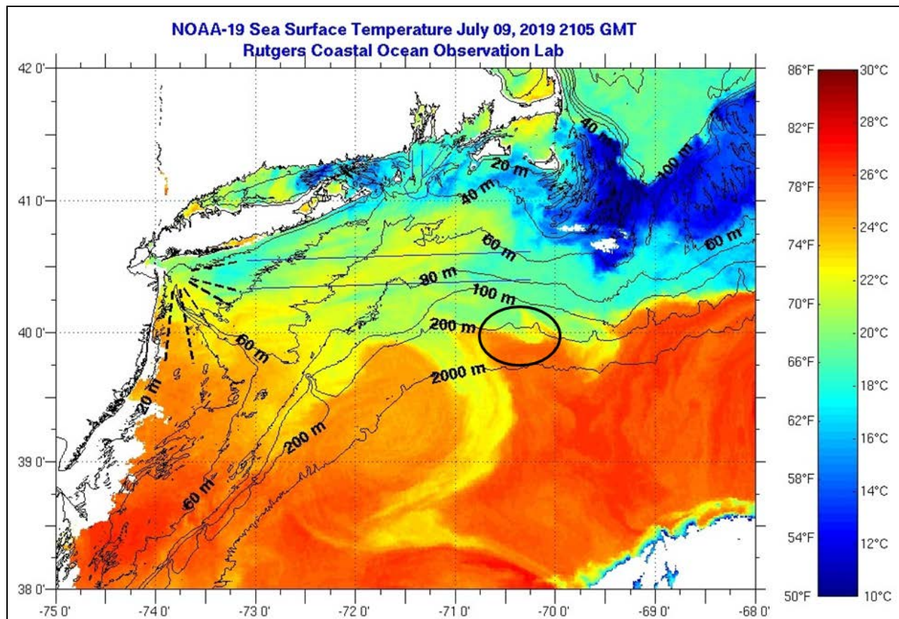
Figure 0712.5. SST on July 9. Black oval indicates the southward meander of the shelf break front observed in the VPR survey shown in Figure 0712.3.
