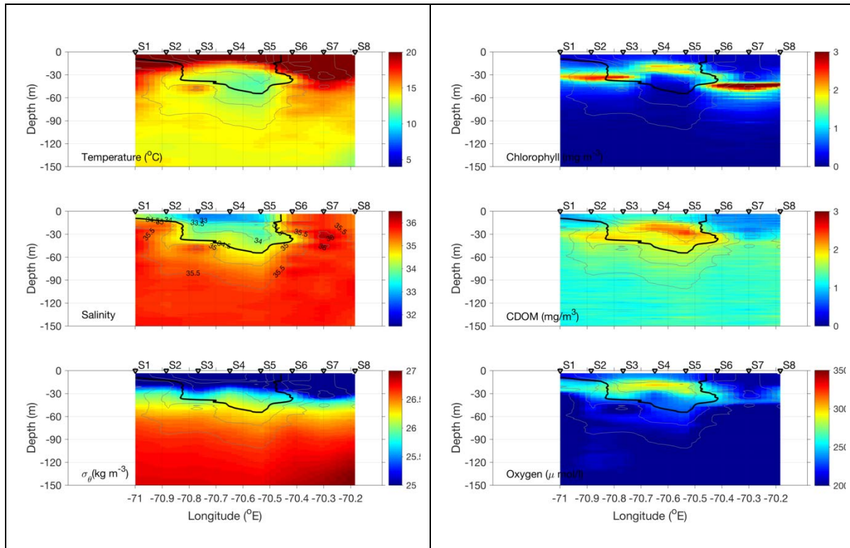
Figure 0708.3. July 8 streamer transect 0-150m.
