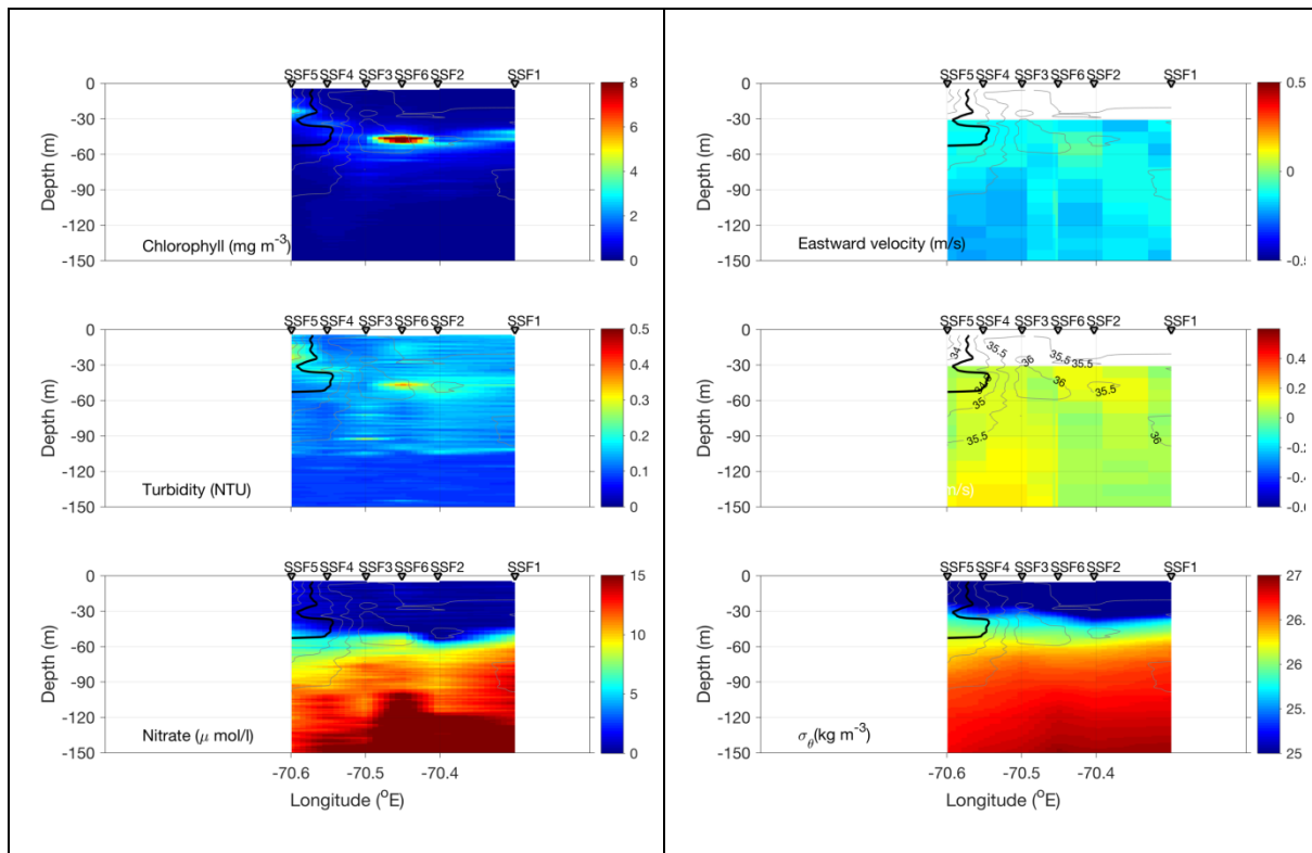
Figure 0710.2. July 10 CTD transect across the streamer/slope front.
