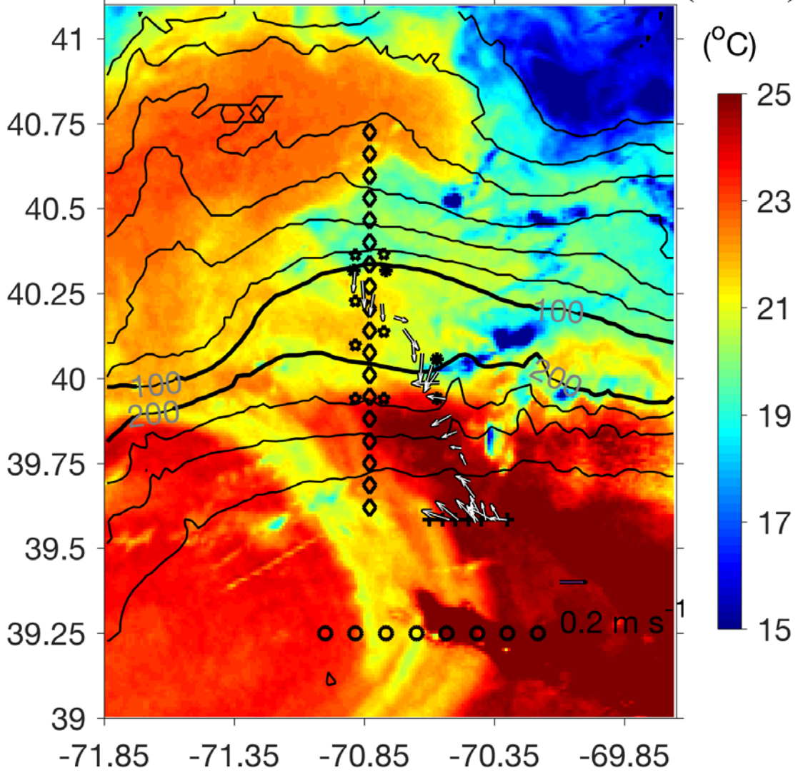
Figure 0710.4. ADCP observation corresponding to the CTD survey (plus signs) shown in Figure 0710.1,2.
