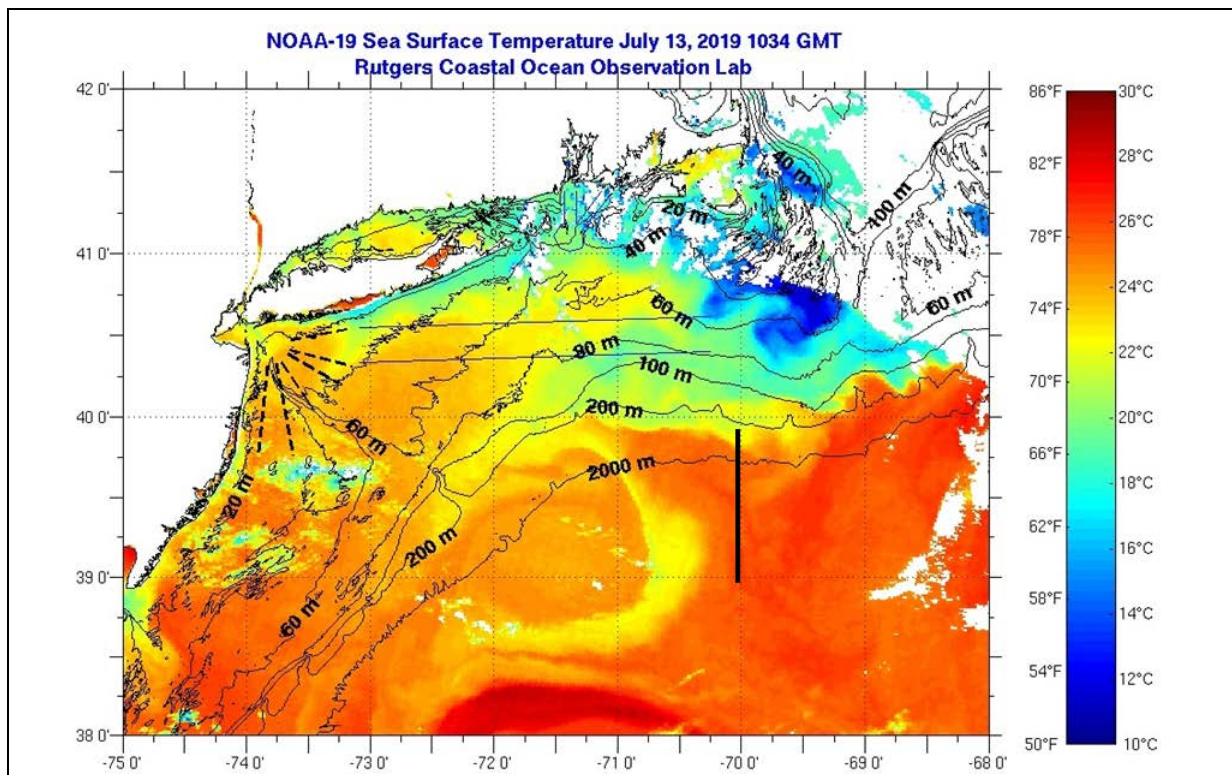
Figure 0715.2. SST on July 13. Approximate location of VPR7 survey shown as a solid line.
