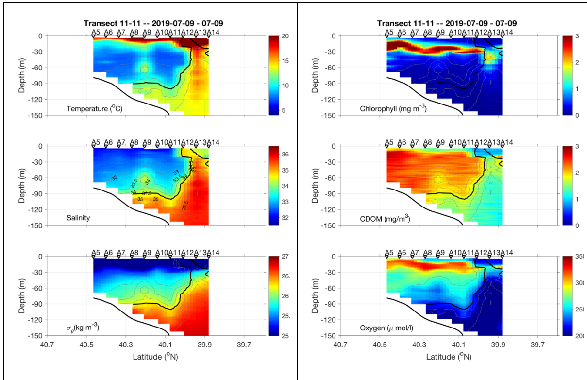
Figure 0709.1. July 9 CTD transect 0-150m.
