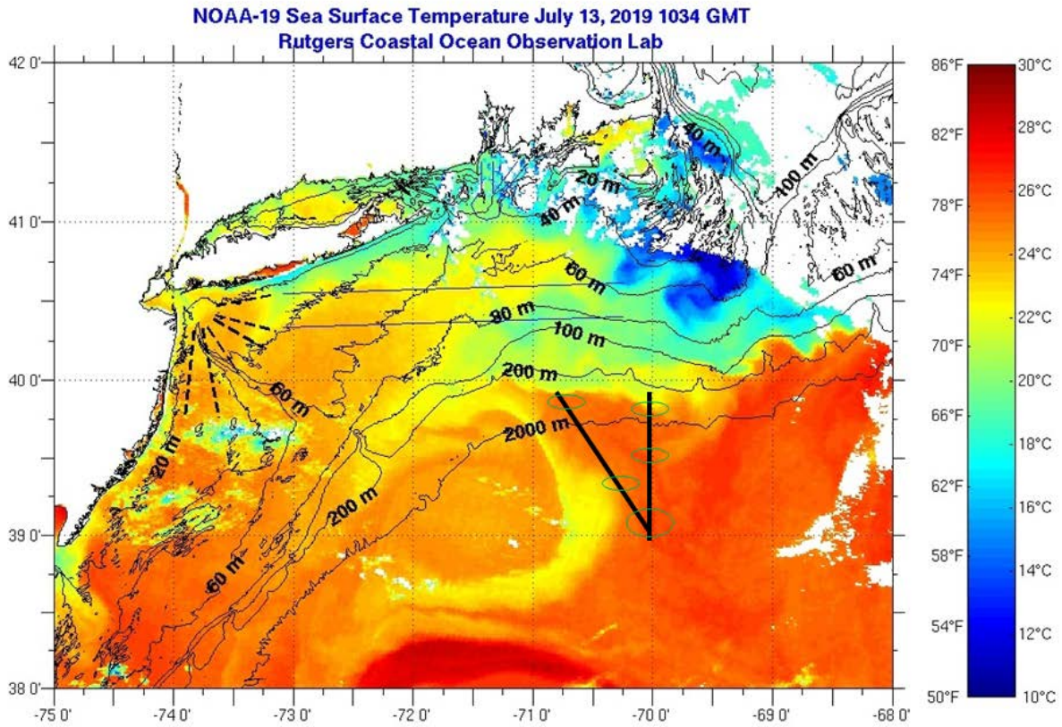
Figure 0715.6. SST on July 13. Approximate location of VPR7/8 surveys shown as a solid line. Green ovals indicate the locations of the five hotspots observed in the fluorescence signal (Figure 0716.5) and VPR imagery.
