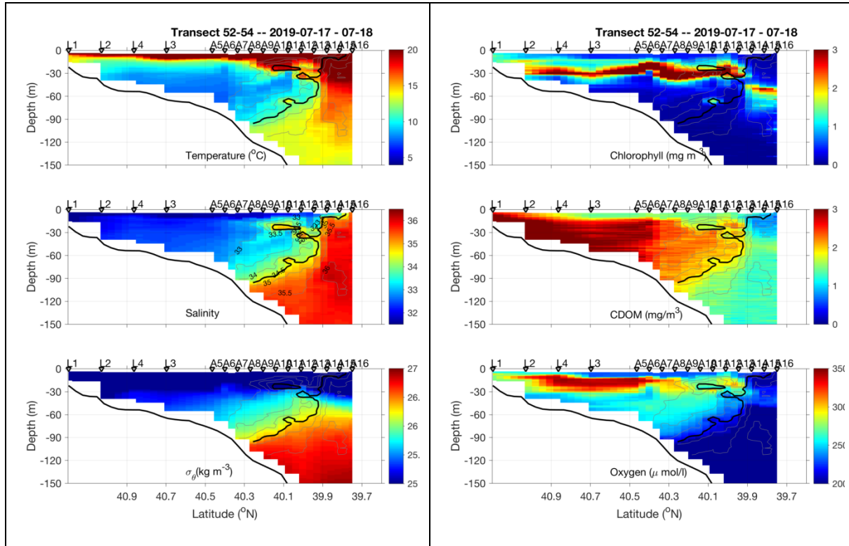
Figure 0718.1. July 17-18 CTD transect. Note labeling of stations L3 and L4 are backward.
