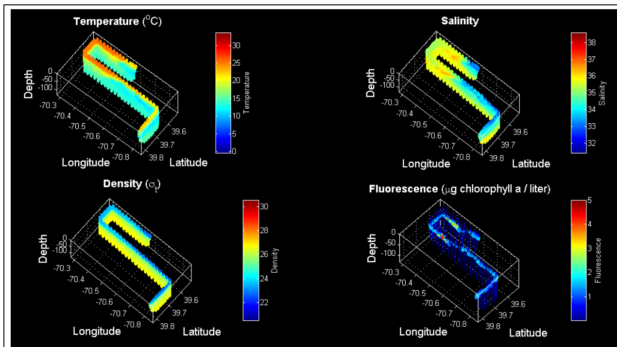
Figure 0709.5. VPR3 July 9, starting from A14 and surveying the diatom population to the east of the streamer.
