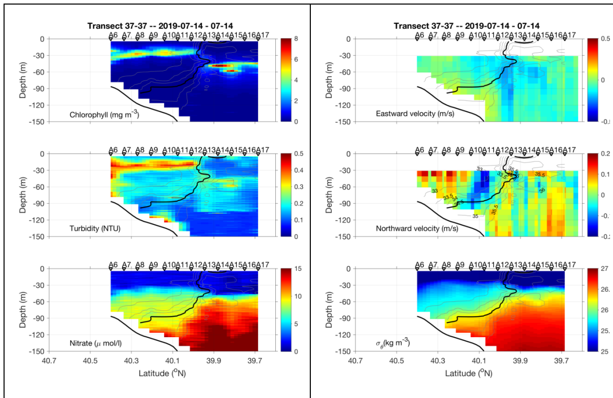
Figure 0714.3. July 14 CTD transect.
