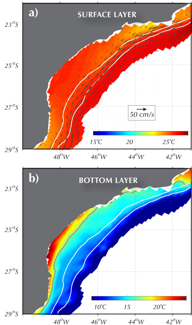
Fig. 4. EXP2: (a) Summer sea surface temperature and surface velocity vectors and (b) Bottom temperature. White contours mark the 100 and 200 isobaths. The black line in panel (b) is the 17 °C isotherm, indicative of the SACW penetration. Note that each panel uses a different color bar.
