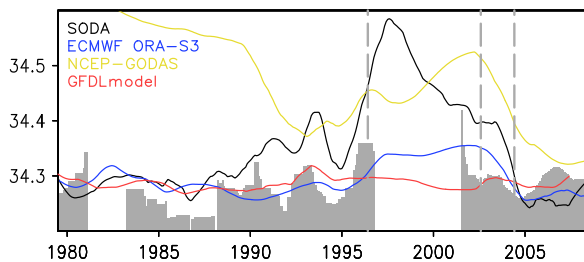
Fig. 6. Time series of the BMC area-mean AAIW ( \sigma = 27.2 ) salinity from the SODA (black), the ECMWF ORAS3 (blue), the NCEP-GODAS (yellow), the GFDL model (red), and the WOD09 in-situ (gray bars) datasets. (For interpretation of the references to color in this figure legend, the reader is referred to the web version of this article.)
