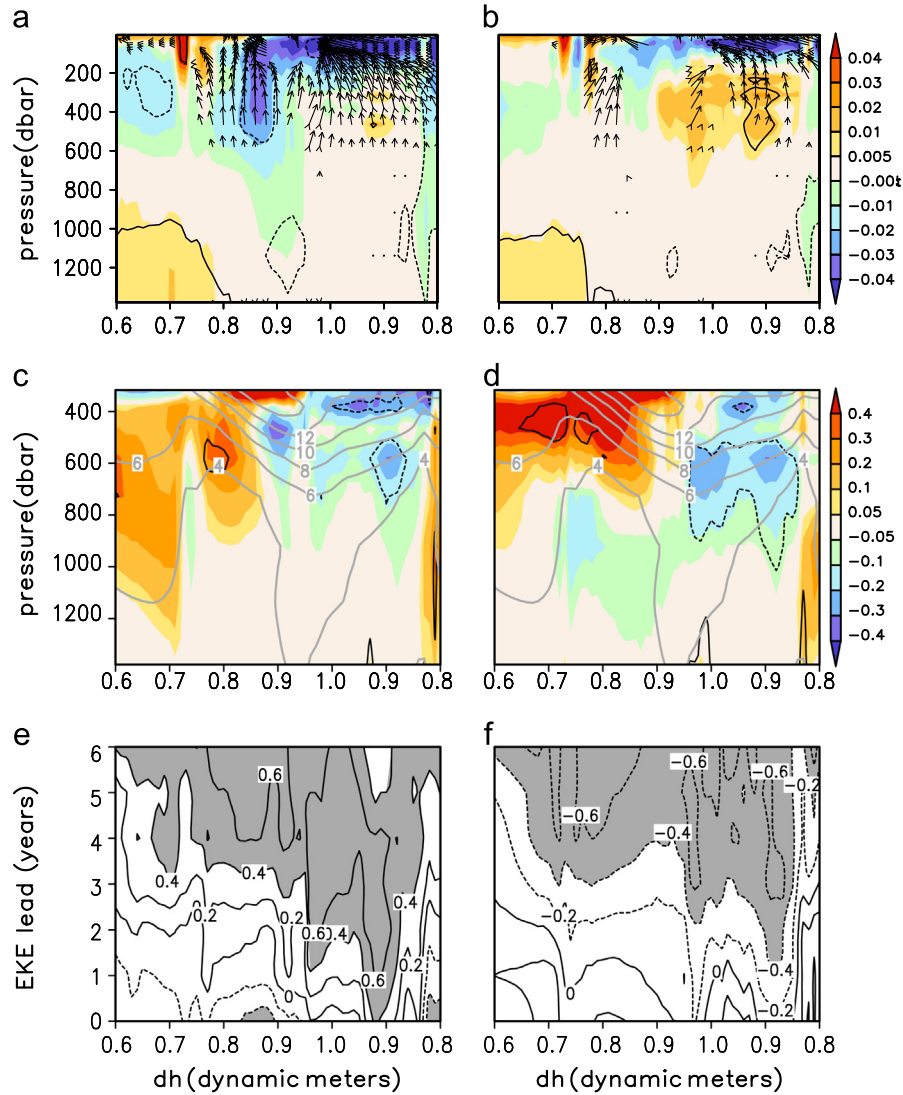
Fig. 4. (a) Dynamic height–pressure section of the regression coefficients of the BMC region along-stream ( 55^{\circ} – 25^{\circ} W mean) potential density (shades, with contours denoting the 95% significance level) and eddy buoyancy flux (vectors, only those vectors above 95% significance level are shown) on SEKEI; (b) same as (a), but for SEKEI leading potential density and eddy buoyancy flux by one year; (c) same as (a), but for SEKEI leading PV by one year, superposing the climatology of potential vorticity (gray contours). The PVs are multiplied by -1 to offset the effect of negative coriolis parameter f on PV values; (d) same as (c), but for SEKEI leading potential vorticity by two years; (e) correlation coefficients between SEKEI and subsurface (465 m) potential density with SEKEI leading by 0 to 6 years (the correlation coefficients above 0.4 are shaded); (f) same as (e), but for SEKEI and PV in intermediate layer (918 m).
