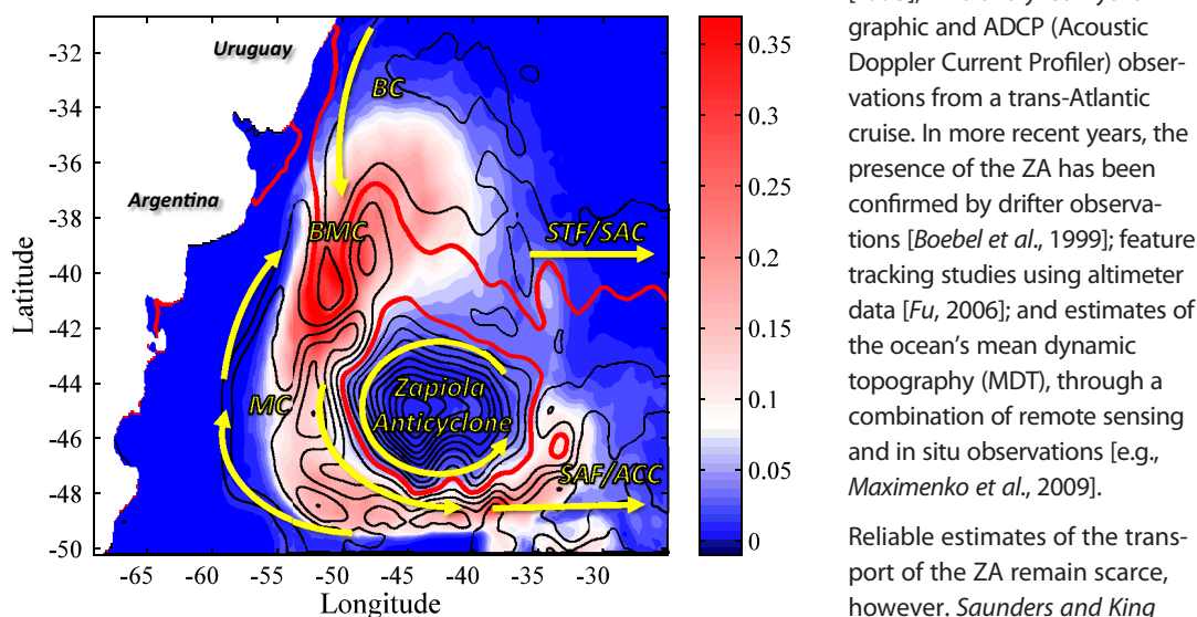
Figure 2. Vertically integrated eddy kinetic energy per unit area (shading; 10^6\text{ kg s}^{-2} ); and distribution of barotropic stream function (contours; interval 25\text{ Sv} , zero-contour in red), as represented by the POP model. Arrows schematically indicate the major flow features, in particular the Zapiola Anticyclone; the Malvinas Current (MC), Brazil Current (BC), and their confluence (BMC); the South Atlantic Current (SAC) and the associated Subtropical Front (STF); and the continuation of the Antarctic Circumpolar Current (ACC) along the Subantarctic Front (SAF).
