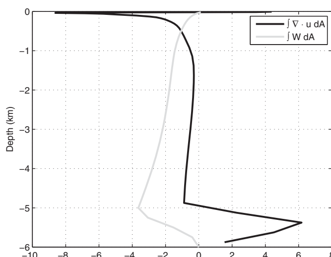
Figure 4. Divergence (black; \text{mSv/m} ) of the horizontal volume flux across the boundary of the Zapiola Anticyclone (defined here as the \Psi=0 contour of the time-mean barotropic stream function in Figure 3). Gray contour shows area-integrated vertical transport (Sv).
