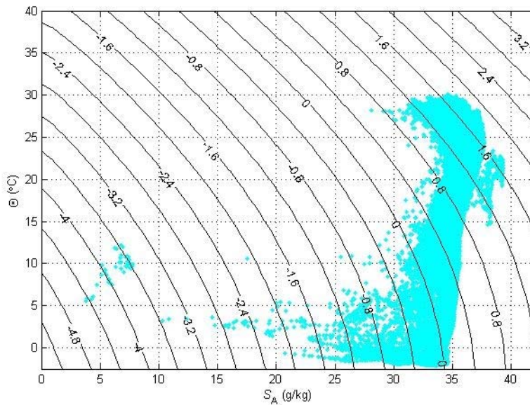
Figure A.14.1. Contours of \left( \frac{|\nabla_n \theta|}{|\nabla_n \Theta|} - 1 \right) \times 100\% at p = 0 , showing the percentage difference between the epineutral gradients of \theta and \Theta . The blue dots are from the ocean atlas of Gouretski and Koltermann (2004) at p = 0 .
