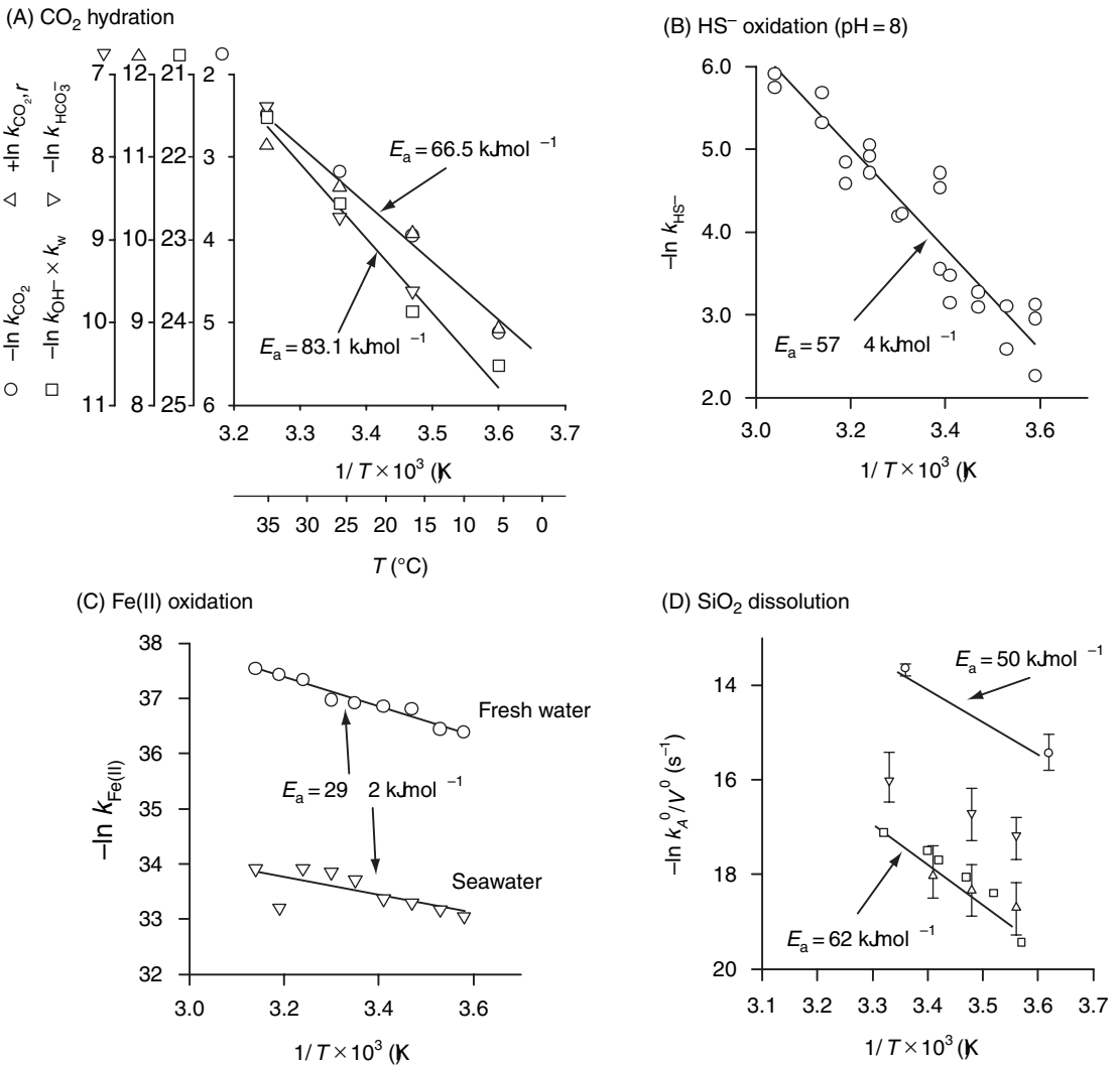
Figure 9.6. Temperature dependence of environmentally important reaction rate constants. (A) CO 2 reaction with H 2 O or OH - in seawater. The data are plotted so that the slope of the line is the Arrhenius activation energy, E_a , divided by the gas constant, R (8.315 J mol -1 deg -1 ) (Johnson, 1982). (B) HS - oxidation (Millero et al. , 1987a). (C) Fe(II) oxidation in seawater (Millero et al. , 1987b). (D) The dissolution rate constants for opal as a function of temperature. The values plotted here are normalized to a constant area: volume ratio, A^0/V^0 = 10 \text{ cm}^{-1} . The high dissolution rate constants (circles) are for acid-cleaned siliceous sediments (Hurd, 1972); the squares are data for peroxide and acid-washed plankton (Lawson et al. , 1978); and the other results (triangles) are for two untreated single species of diatom (Kamatani, 1982).
