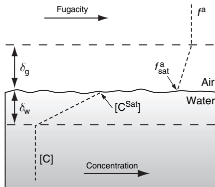
Figure 10.2. A schematic diagram of the stagnant molecular layers of thickness \delta_g and \delta_w near the air–water interface. Fugacity in the bulk atmosphere and water are indicated by f^a and [C] , respectively. Chemical equilibrium at the air–water interface is described by Henry’s Law, where K_H f_{sat}^a = [C^{Sat}] .
