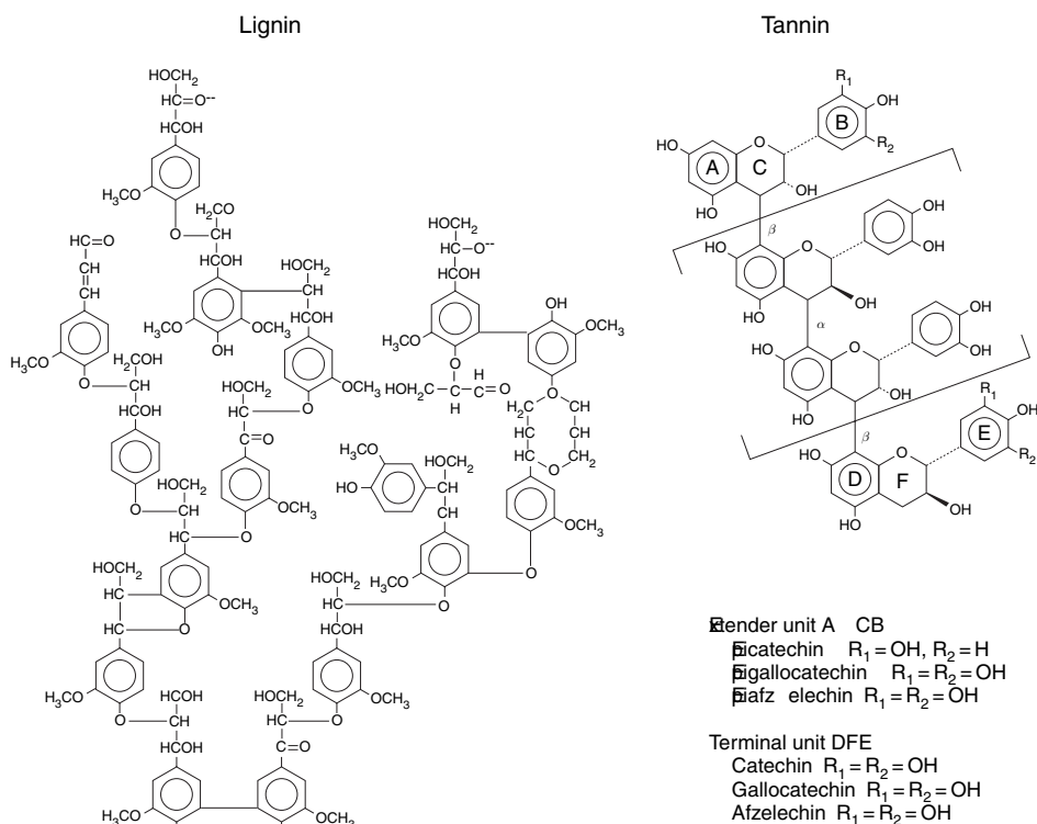
Figure 8.16. Schematic chemical structures of lignin and tannin polyphenols. The benzene ring of lignin structural units can be substituted by 0, 1 or 2 methoxyl ( -\text{OHC}_3 ) groups, in positions flanking the phenolic hydroxyl group. The extent of substitution is related to the taxonomy of vascular plants. The structure of condensed tannin is shown here along with its building blocks of three-ring flavonols (see figure for terminology of extender and terminal units). Several variations of these stereochemically active compounds occur in condensed tannin.
