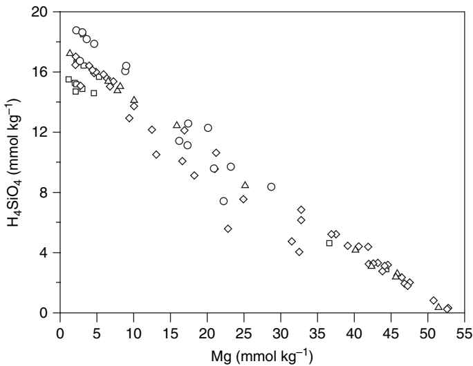
Figure 2.10. | \text{H}_4\text{SiO}_4 and \text{Mg}^{2+} concentrations measured in the neck of a “hot smoker” at the East Pacific Rise at the 21° N hydrothermal area in the North Pacific Ocean. Symbols indicate data from different vents. The range of concentrations varies from the seawater end member on the right-hand side with 53 mmol kg -1 \text{Mg}^{2+} and near zero \text{H}_4\text{SiO}_4 to the “hydrothermal end member” with near zero \text{Mg}^{2+} concentration and between 16 and 20 mmol kg -1 \text{H}_4\text{SiO}_4 . From Von Damm et al. (1985).
