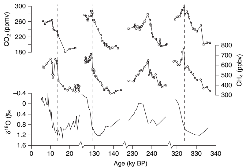
Figure 7.18. The four glacial–interglacial transitions over the past 400 ky in the Vostok ice core, showing the relations among the gases \text{CO}_2 , \text{CH}_4 and \delta^{18}\text{O}\text{-O}_2 in the bubbles of the ice core. Vertical dashed lines are drawn through the “jumps” in the \text{CH}_4 concentrations. These data illustrate the temporal relations between the changes in atmospheric chemistry and ice volume change (see text). Redrawn from Petit et al. (1999).
