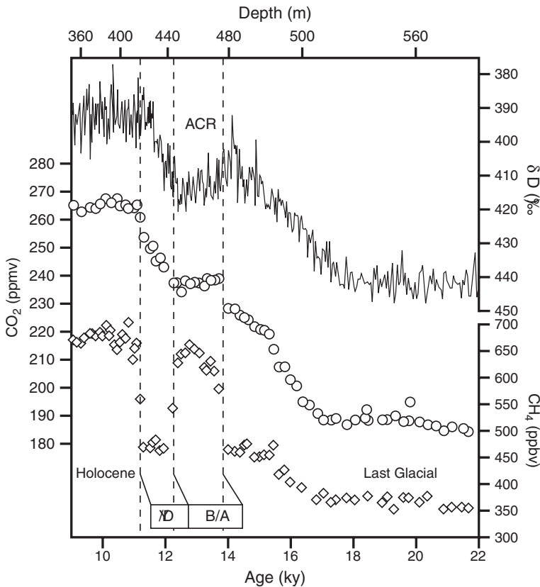
Figure 7.20. Temperature proxy ( \delta D ) and gas concentrations in bubbles from the Dome C ice core in Antarctica ( 75^{\circ}06' S, 123^{\circ}24' E ) during the last glacial–interglacial transition. The Younger Dryas (Y/D) and Bølling/Allerød (B/A) events recorded in the Greenland ice cores are also present in Antarctic ice and are indicated according to the Greenland GRIP ice core time scale. CH_4 is a global atmospheric signal; similar CH_4 changes are observed at both poles. However, changes in temperature and CO_2 during the B/A and Y/D periods indicated here are in the opposite sense from those observed in Greenland. The ice age – gas age difference between the \delta D and gas records is based on an ice accumulation model. Redrawn from Monnin et al. (2001).
