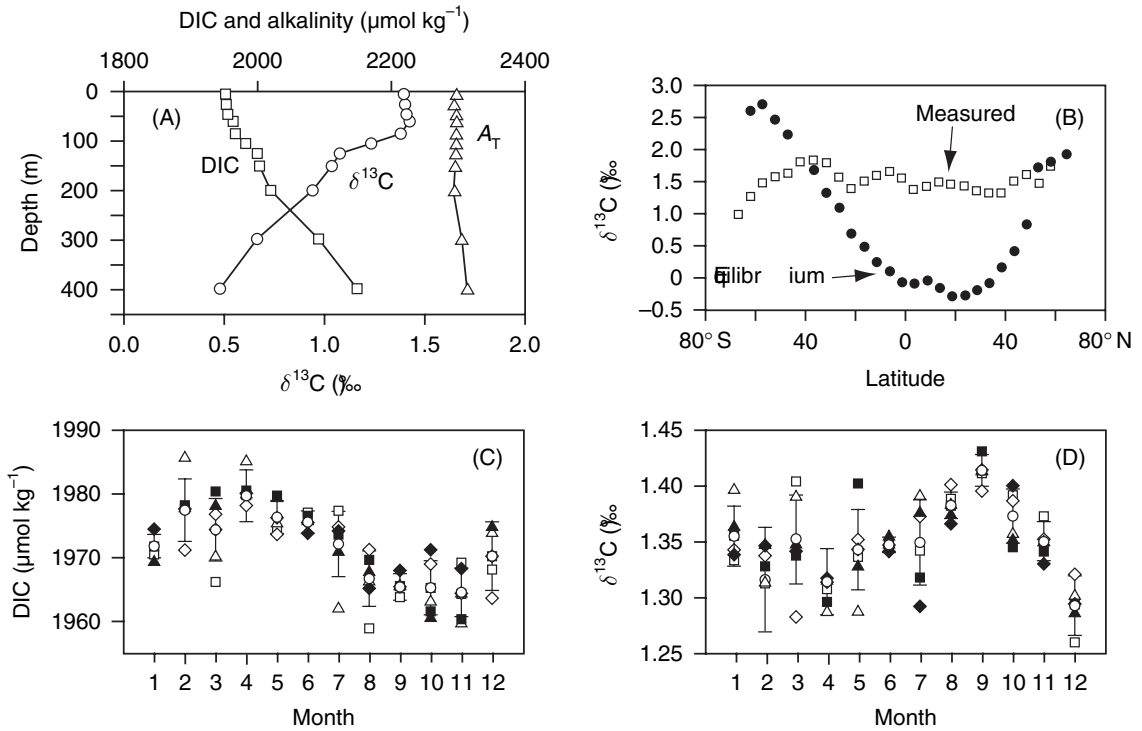
Figure 6.14. DIC and carbon isotope ratio of DIC, \delta^{13}\text{C} -DIC, in the North Pacific Ocean. The depth and time series data are from the Hawaii Ocean Time series (HOT) between 1994 and 1999. (A) Depth profile of DIC (squares), total alkalinity, A_T (triangles) and \delta^{13}\text{C} -DIC (circles). (B) Zonally averaged mean values of the surface water \delta^{13}\text{C} -DIC in the Pacific Ocean (squares) and the \delta^{13}\text{C} -DIC expected if the surface ocean DIC were in chemical equilibrium with the atmosphere (circles). (C) Monthly values of DIC in the mixed layer at HOT. (D) Monthly values of \delta^{13}\text{C} -DIC in the mixed layer at HOT. Redrawn from Quay and Stutzman (2003).
