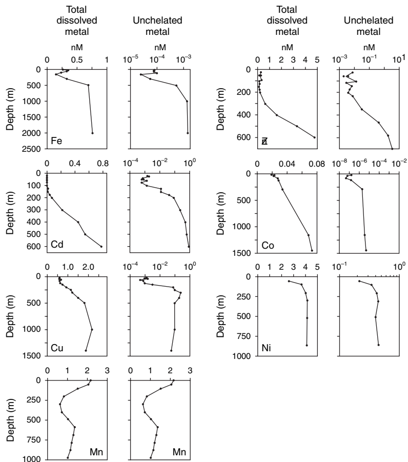
Figure 6.4. Fe, Mn, Co, Cu, Zn, Ni and Cd profiles as a function of depth in the oceans. Profiles in the left graph for each element are total metal concentration (the horizontal axis is linear). The profiles on the right are concentrations that are unchelated by organic metal complexes. This includes the free metal ion and all inorganic complexes. Notice that the horizontal axis for the graphs of unchelated metals is logarithmic (except for Mn). Redrawn from Morel et al. (2003).
