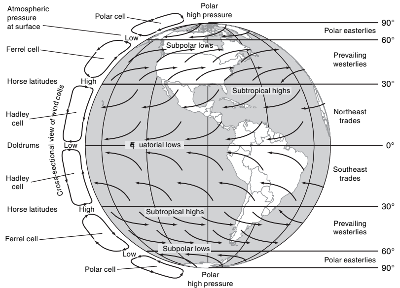
Figure 1.8. The latitudinal distribution of the wind directions on the Earth's surface. (Redrafted from Pinet (1994).)
