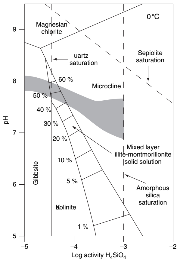
Figure 2.6. A \text{pH} - \rho\{\text{H}_4\text{SiO}_4\} thermodynamic stability diagram among some of the major silicate mineral phases on the Earth's surface. The gray area is the location of seawater pH and silicate concentration. Notice that the minerals predicted to be stable are those enriched in cations, such as the mixed-layer illite–montmorillonite clay minerals and microcline, rather than the less cation-rich kaolinite. The percent scale is the relative mixture of illite in the illite–montmorillonite solid solution. From Helgeson and Mackenzie (1970).
