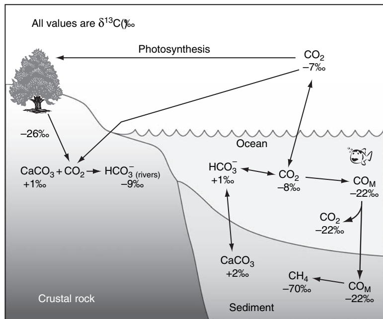
Figure 5.6. Schematic diagram of the exchanges and stable carbon isotope ratios among the reservoirs of atmospheric \text{CO}_2 , ocean \text{HCO}_3^- and \text{CO}_2 , solid organic carbon ( \text{C}_{\text{OM}} ) and \text{CaCO}_3 and \text{CH}_4 . Numbers under the chemical symbols represent the isotopic ratio in ‰. See Table 5.3 for an estimate of the fractionation factors.
